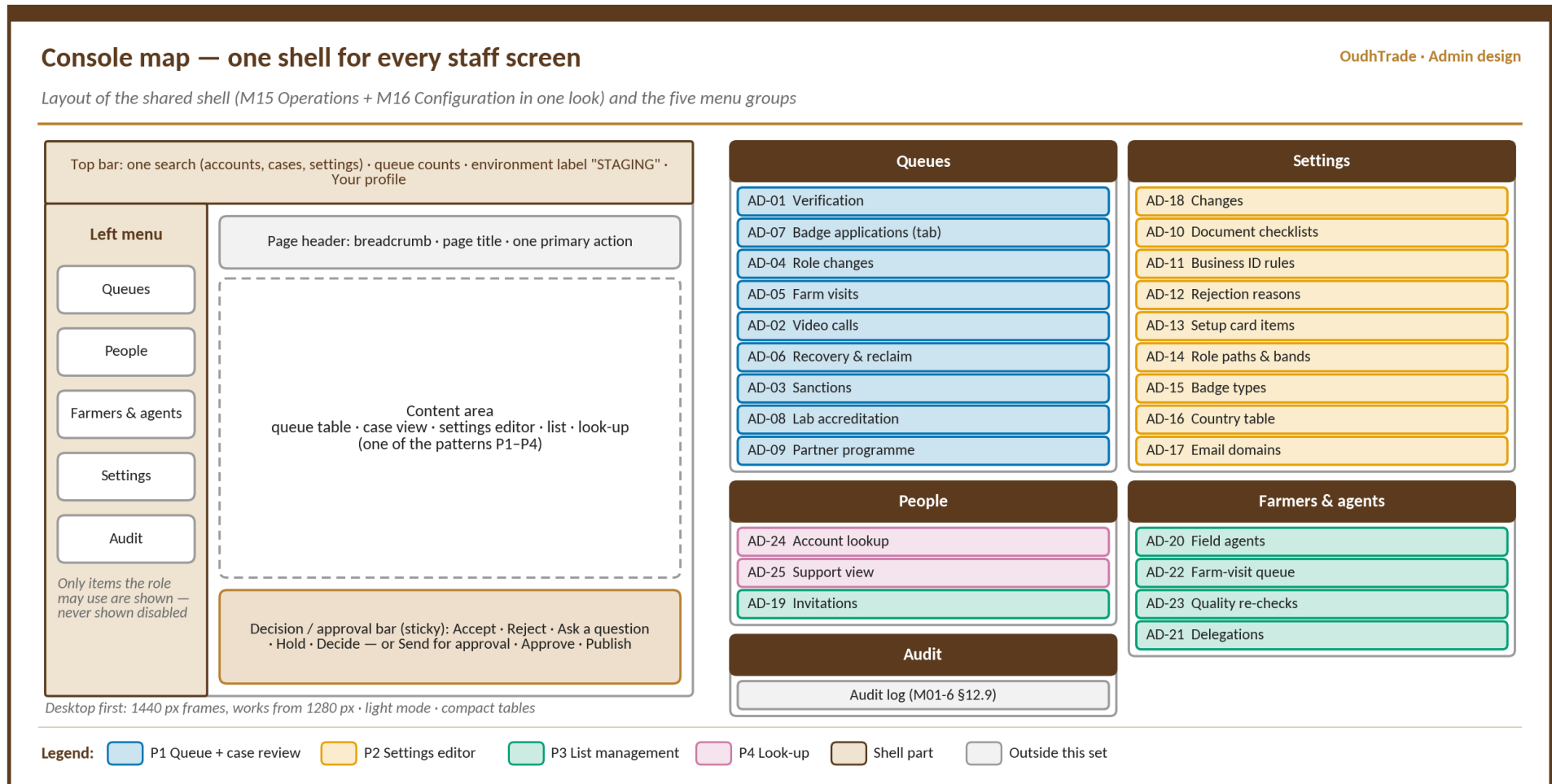
Figure 2 — Console shell and the five menu groups
