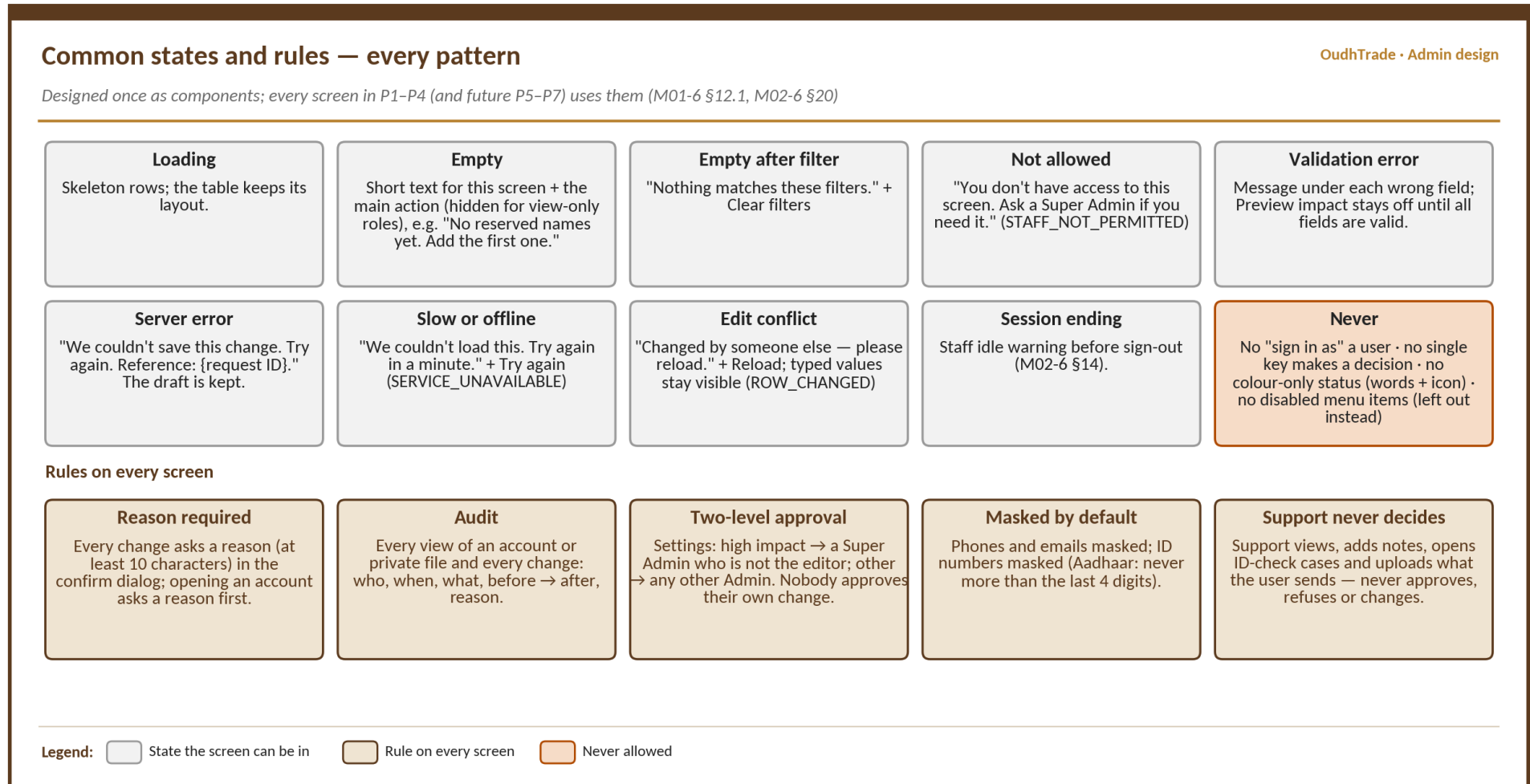
Figure 9 — Common states and rules for all patterns
